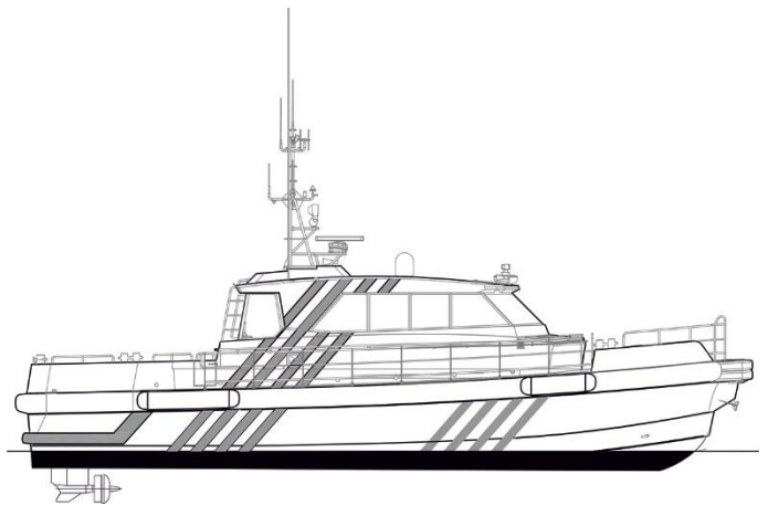
GENERAL ARRANGEMENT SC AMETHYST
